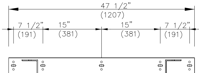
Rail Bracket Dimensions
