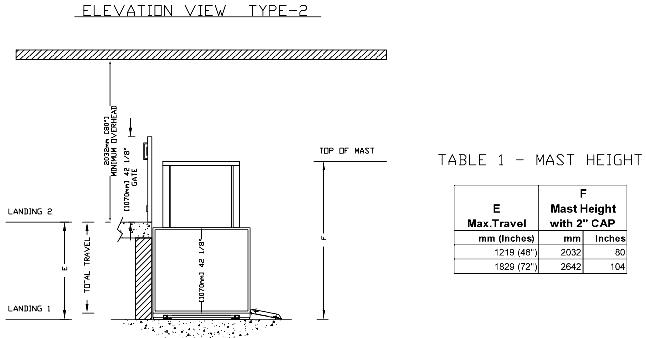
Figure 21: Elevation and plan view – type 2 with platform gate – 42" x 48", 42" x 54", 42" x 60"
