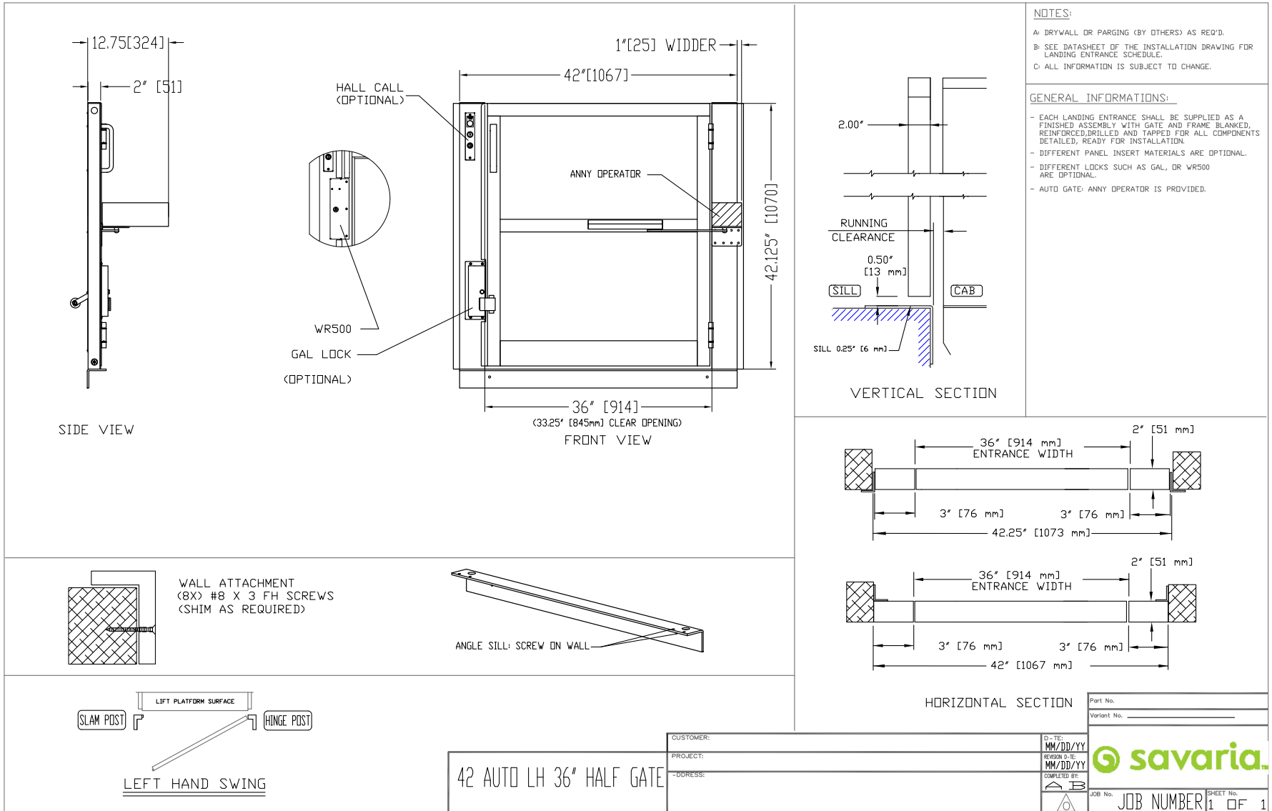
Figure 32: Auto half gate, left-hand
