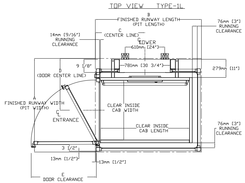
Figure 18: Elevation and plan view, enclosure application (Type 1L)
