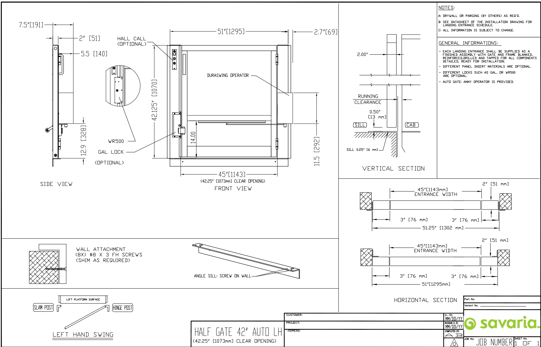
Figure 39: DuraSwing on half gate, left-hand, 45" opening
