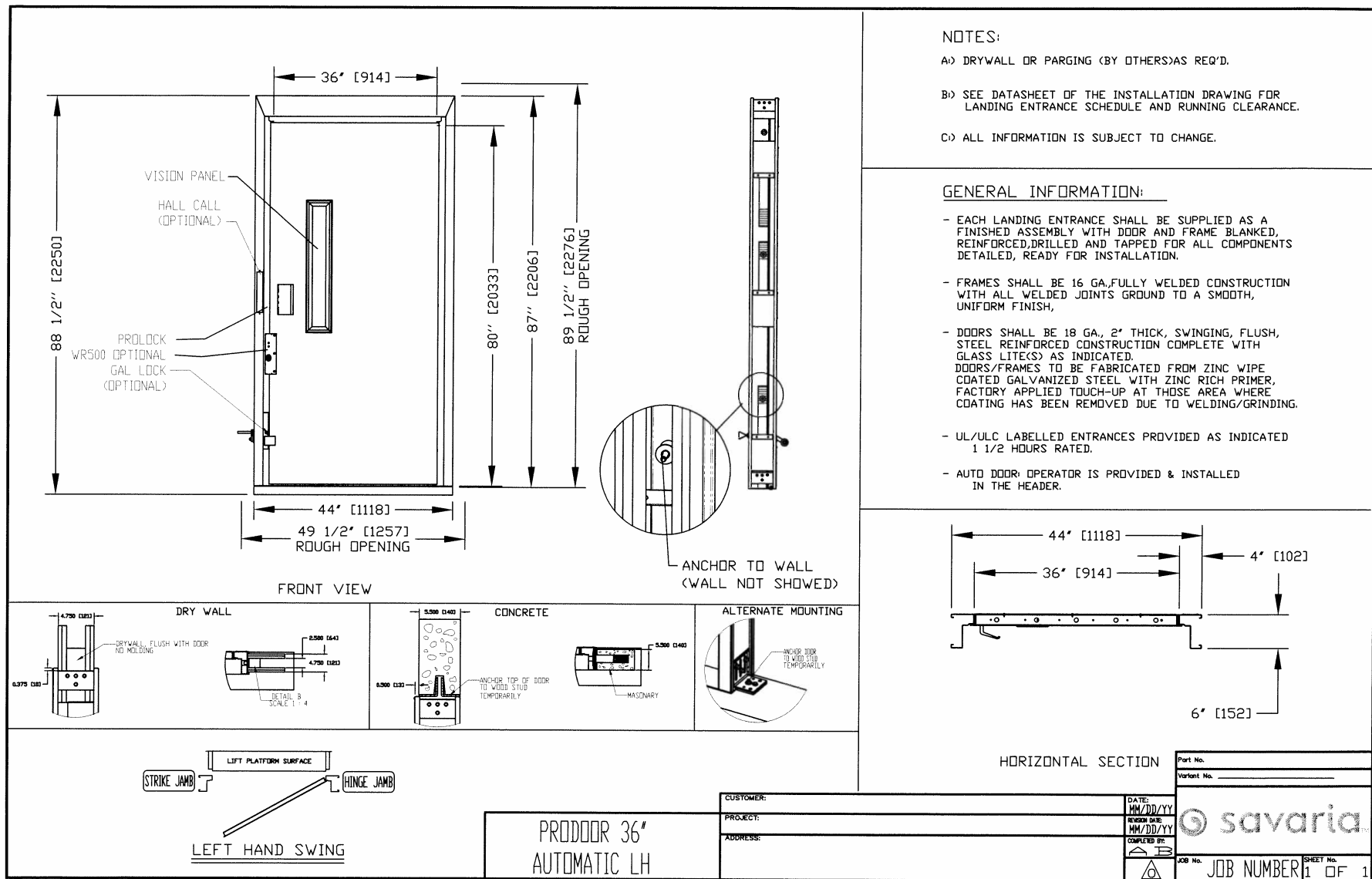
Figure 27: Prodoor auto, left-hand
