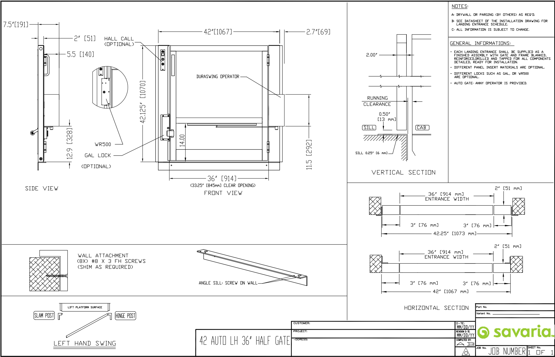
Figure 38: DuraSwing on half gate, left-hand
