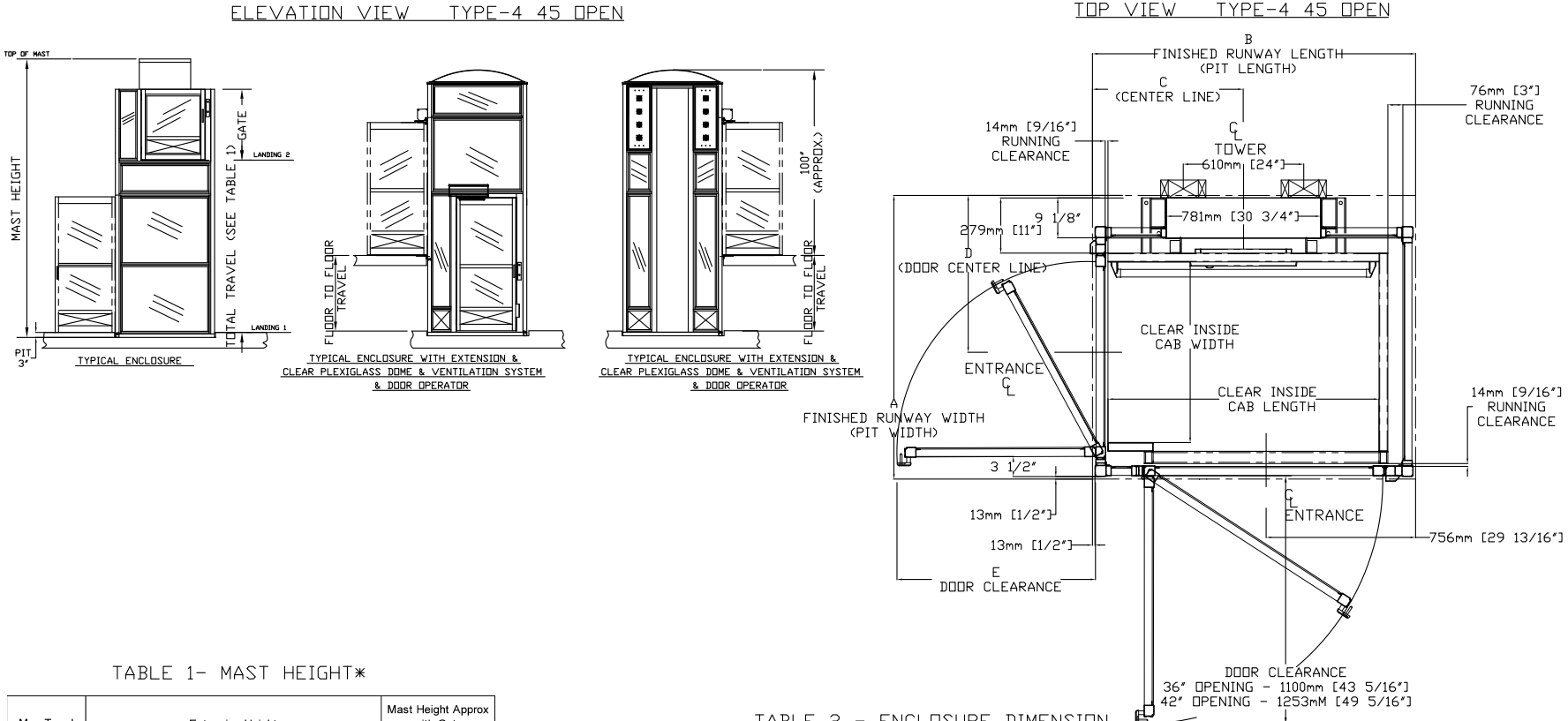
Figure 22: Elevation and plan view, enclosure application (Type 4, 45" opening)
