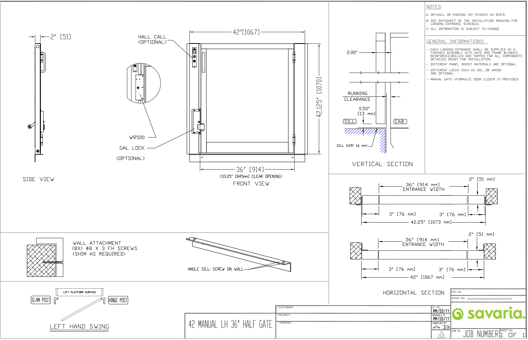
Figure 34: Manual half gate, left-hand
