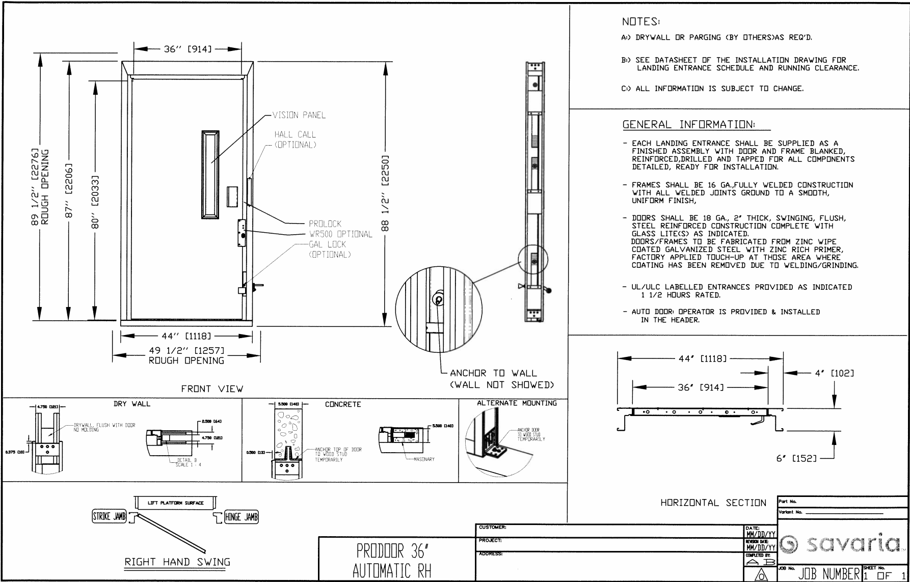
Figure 28: Prodoor auto, right-hand
