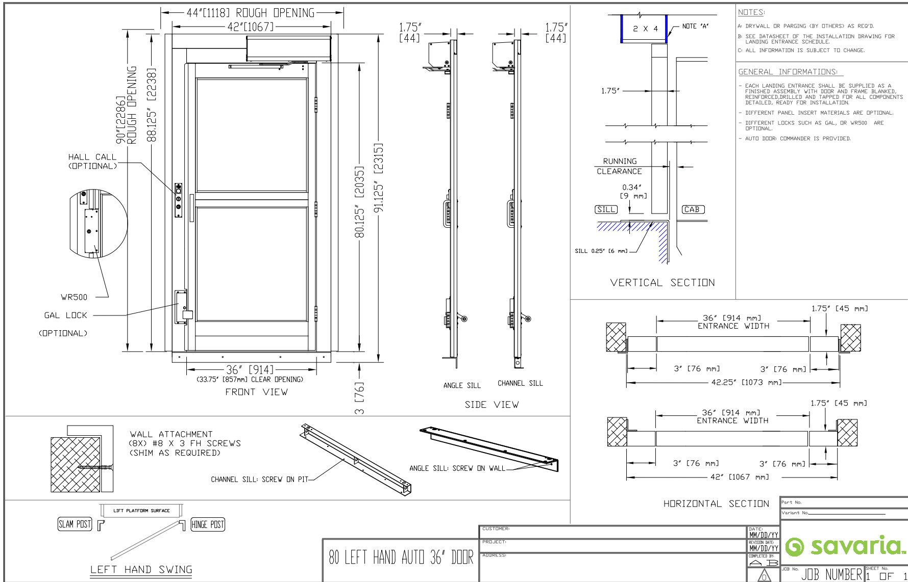
Figure 23: Auto door, left-hand
