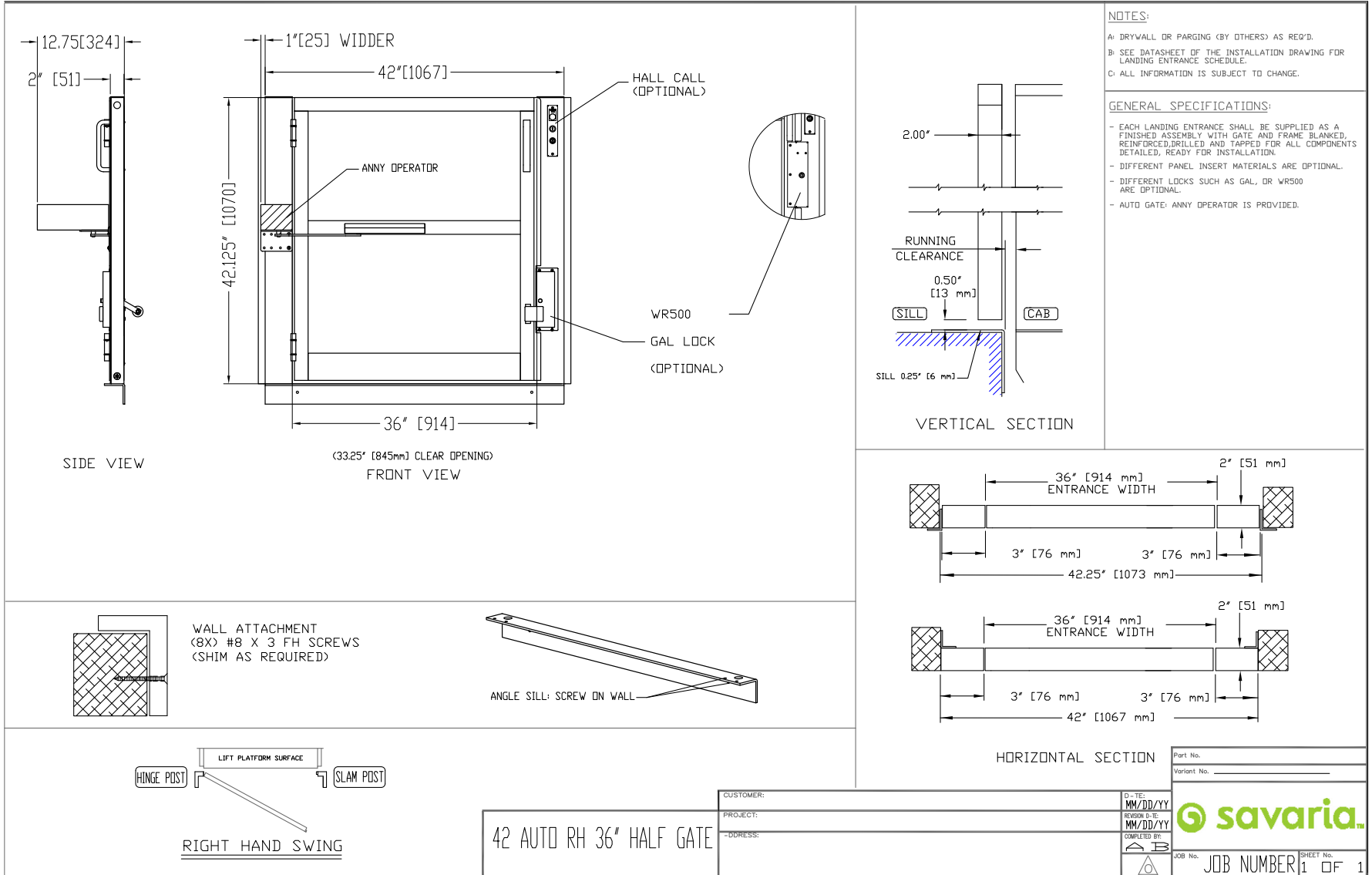
Figure 33: Auto half gate, right-hand
