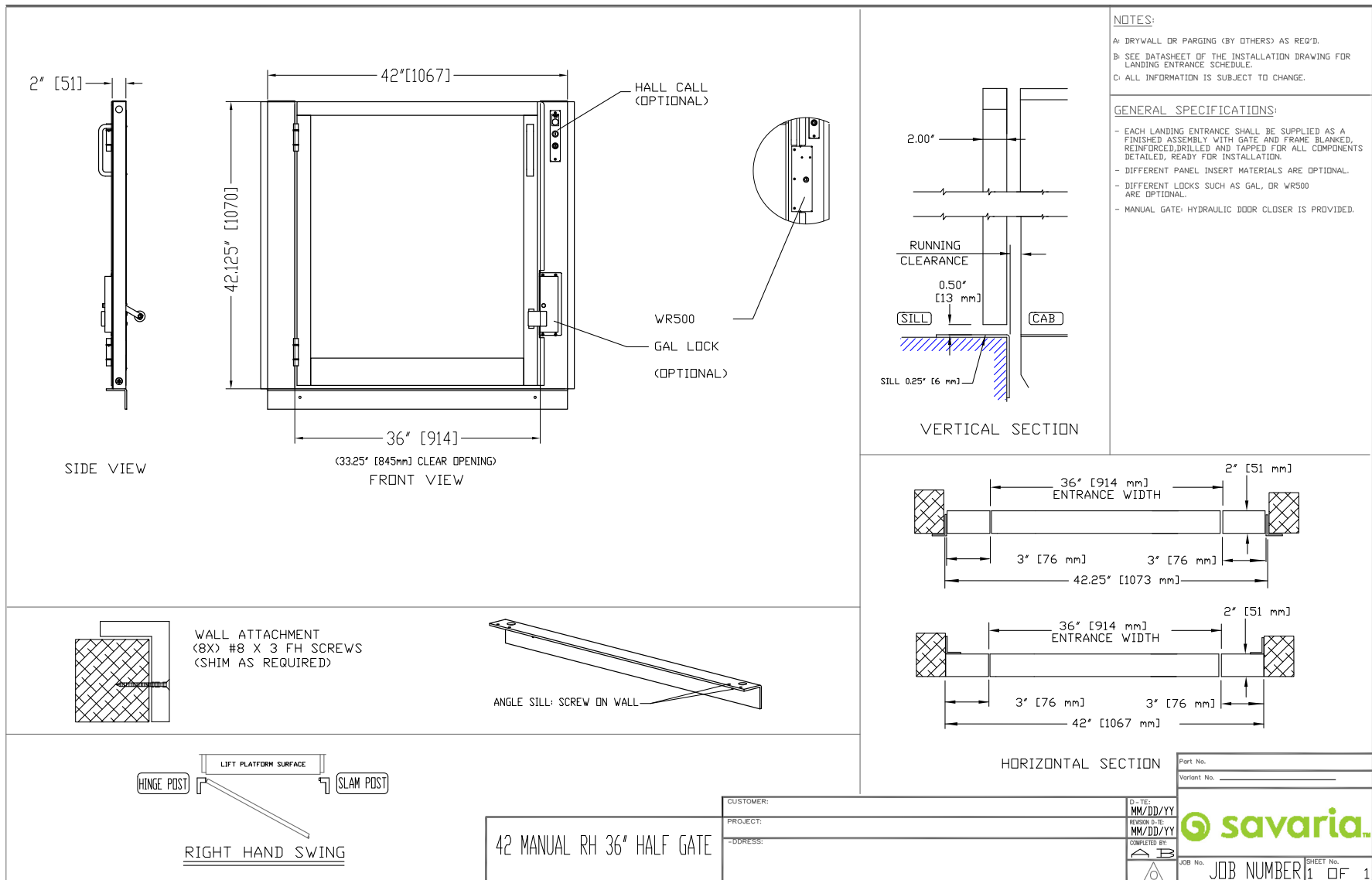
Figure 35: Manual half gate, right-hand
