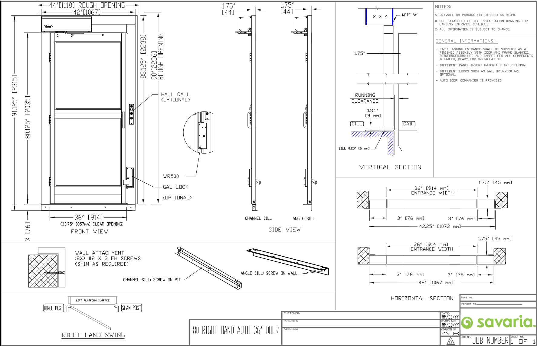
Figure 24: Auto door, right-hand
