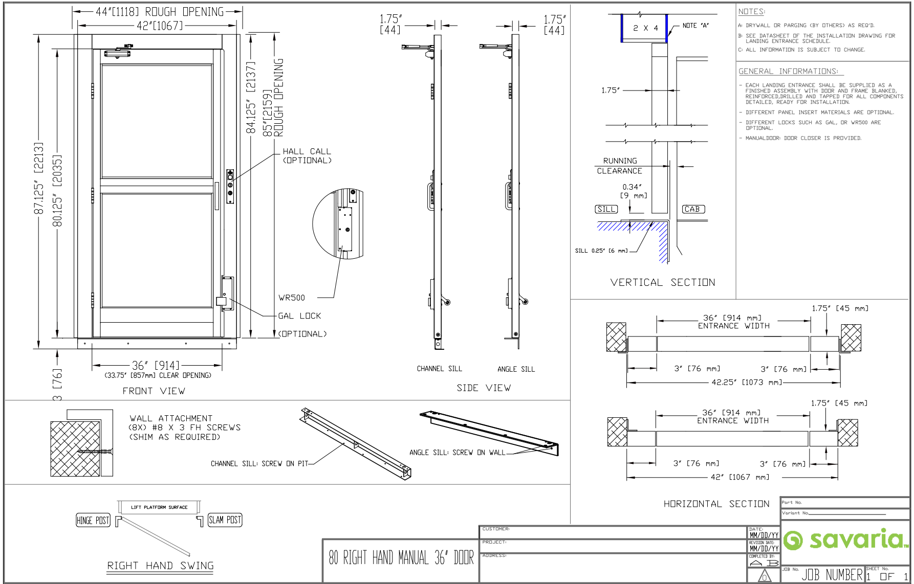
Figure 26: Manual door, right-hand
