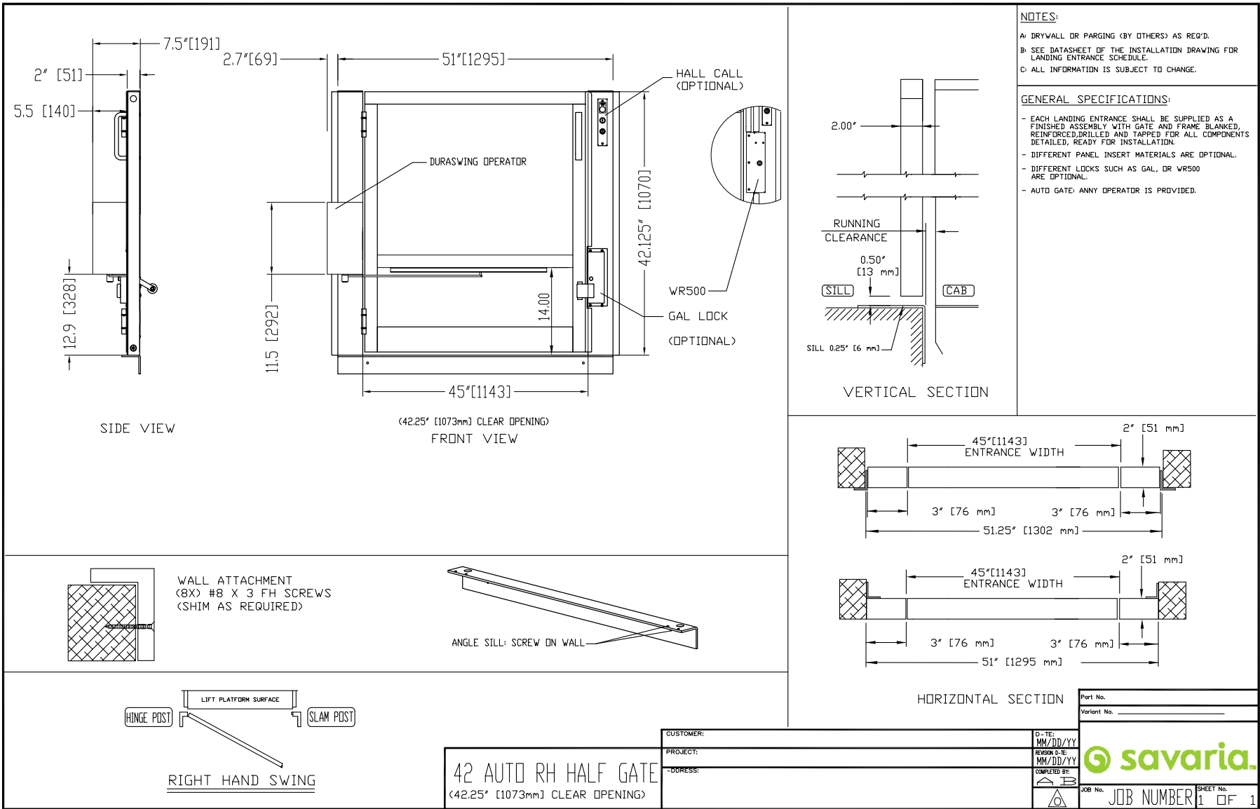
Figure 37: DuraSwing on half gate, right-hand, 45° opening
