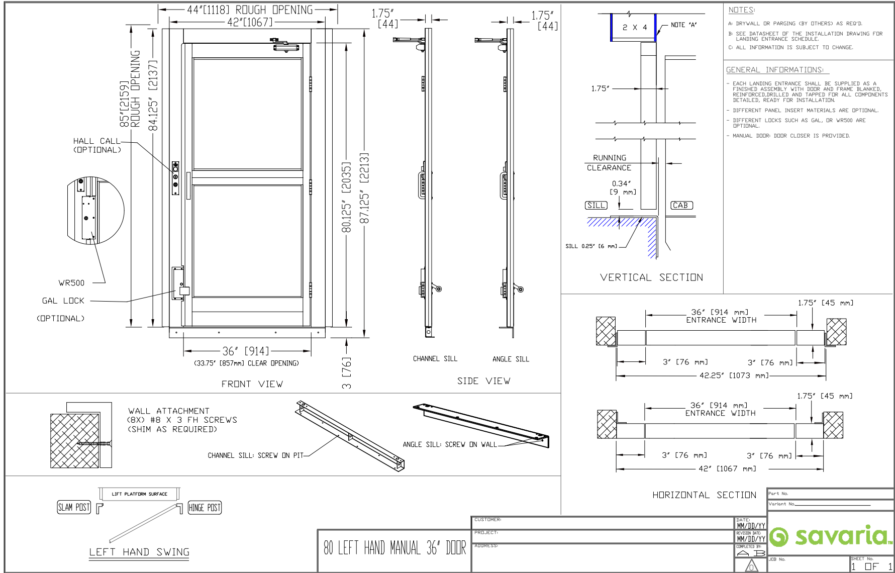
Figure 25: Manual door, left-hand
