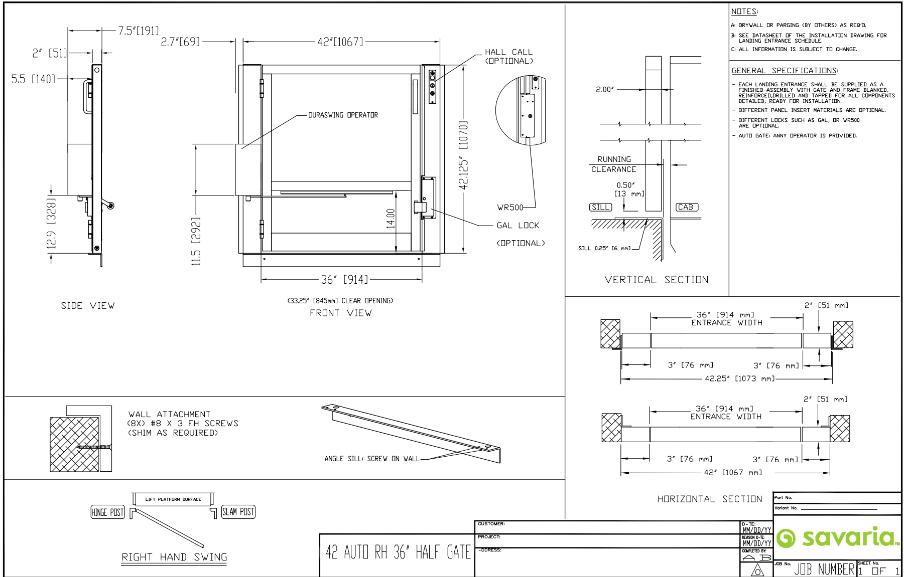
Figure 36: DuraSwing on half gate, right-hand
