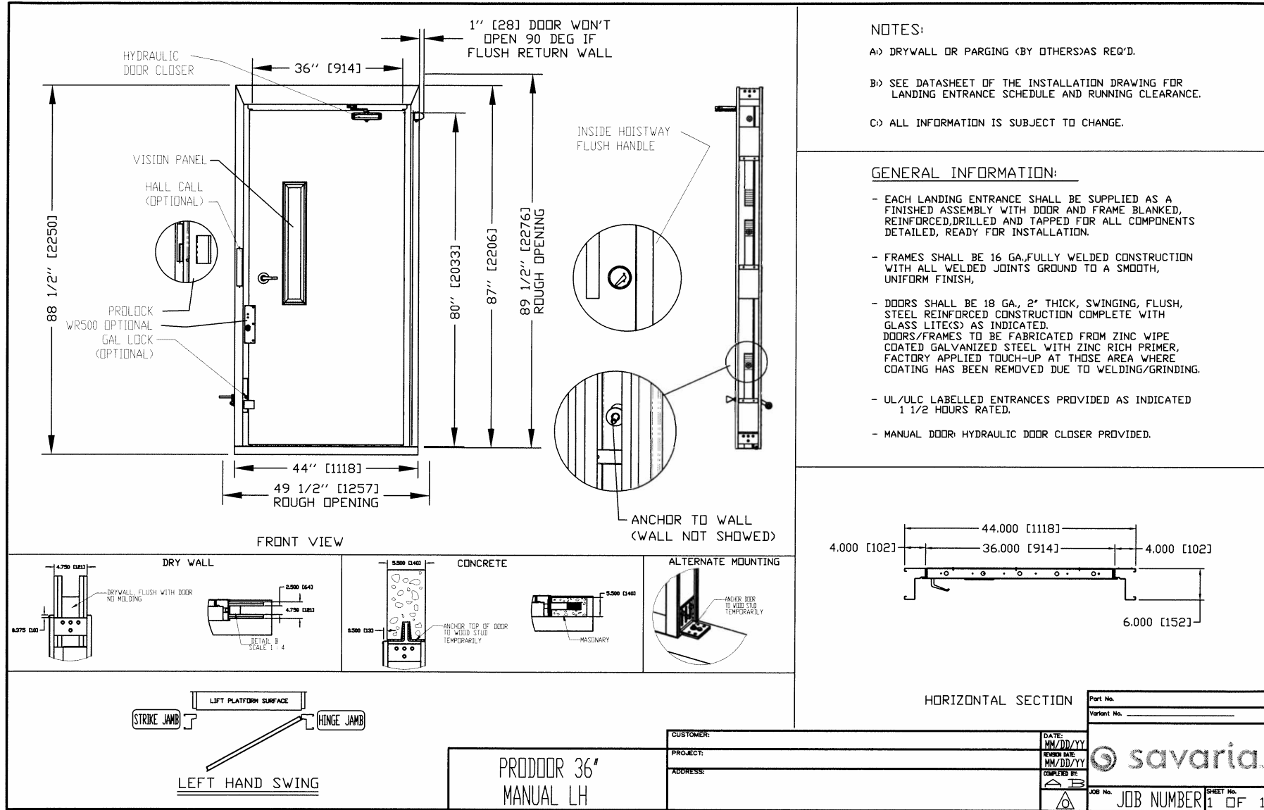
Figure 29: Prodoor manual, left-hand
